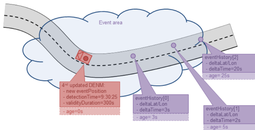
Figure 2 (h) - Generation and evolution of eventHistory along an event area
